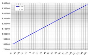
curve Pt1000
